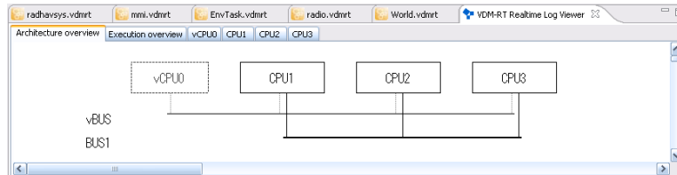
Figure 3.11: Architectural overview
