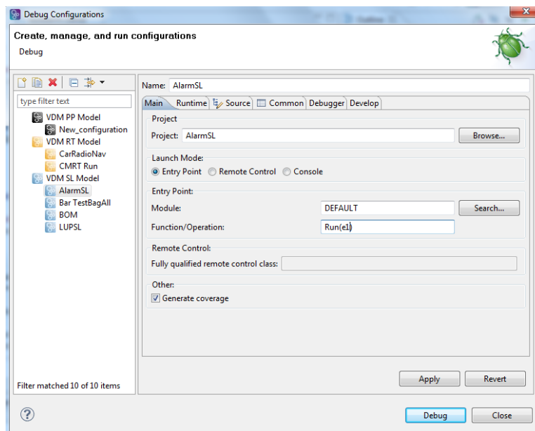
Figure 3.9: The debug configuration dialog
