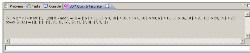
Figure 3.5: The VDM quick interpreter view
