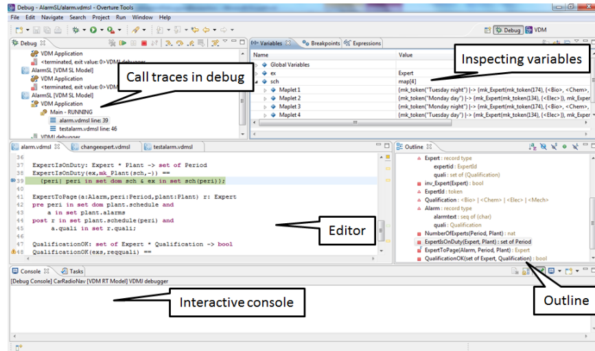
Figure 3.10: Debugging perspective
